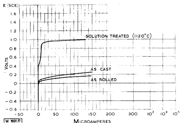
Fig. 17. Effect of solution treatment on polarisation characteristics in 3% NaCl – composition 25Cr5Ni3Cu2.5Mo – temp. 30 °C – N 2 purged
