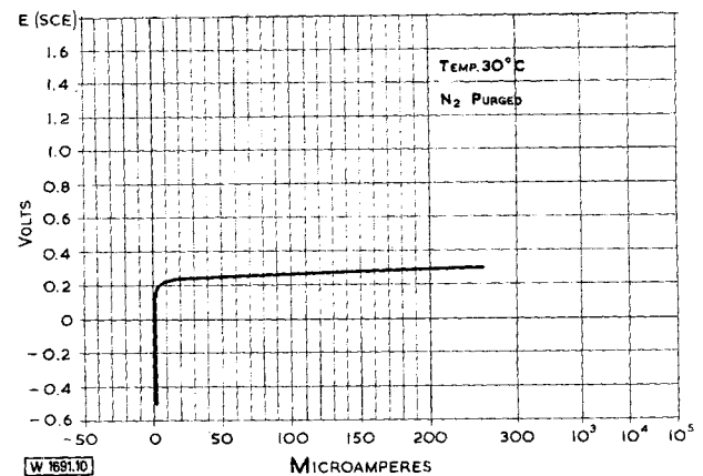
Fig. 10. Polarisation characteristics of 18Cr10Ni3Mo in 3% NaCl
