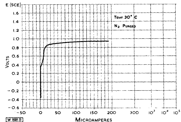
Fig. 11. Polarisation characteristics of Ferralium alloy in 3% NaCl
